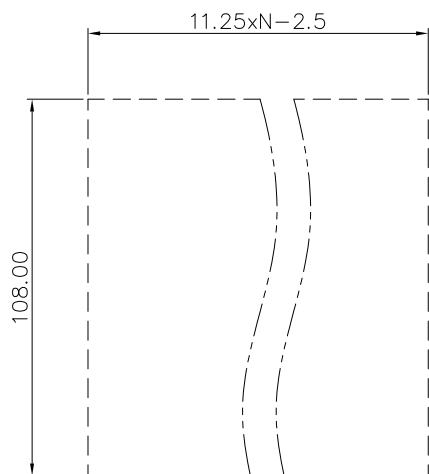
PCB LAYOUT
